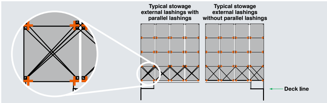
CONTAINERS SECURED BY TWISTLOCKS AND LASHING RODS, 'EXTERNAL LASHING' ARRANGEMENT
