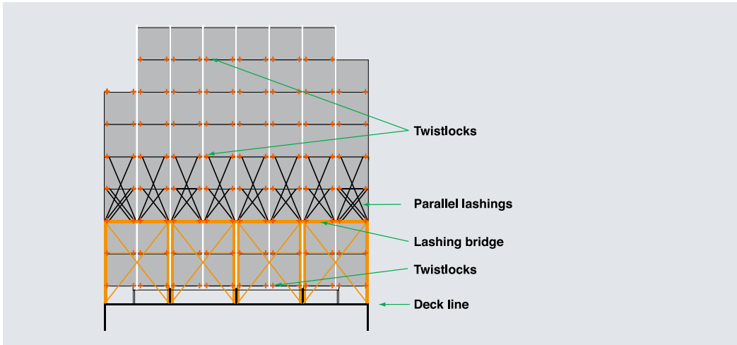
AS ABOVE BUT LASHINGS ORIGINATE FROM A LASHING BRIDGE. LASHING RODS TO BOTTOM OF FIFTH TIER
