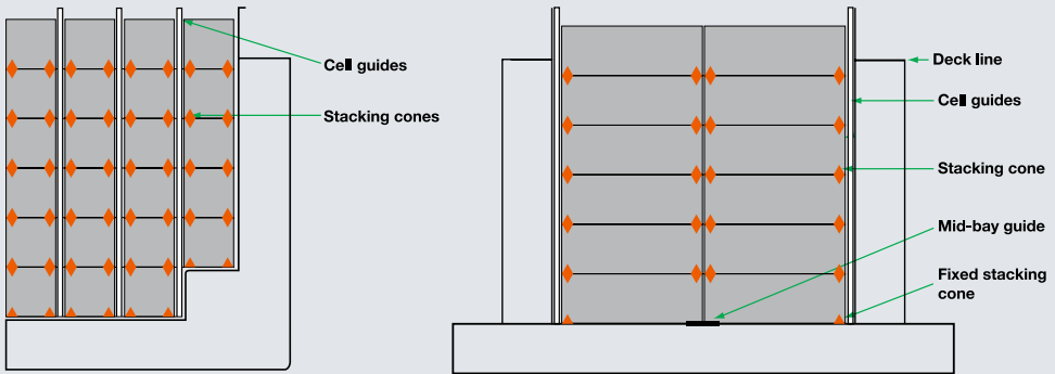
20-FOOT CONTAINERS IN 40-FOOT CELL GUIDES
