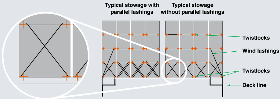
CONTAINERS SECURED BY TWISTLOCKS AND LASHING RODS. LASHING RODS TO BOTTOM OF SECOND TIER. WIND LASHINGS TO BOTTOM OF THIRD TIER
