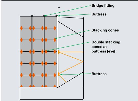
TYPICAL BULK CARRIER STOWAGE ARRANGEMENT WITH BUTTRESSES, USING SINGLE/DOUBLE STACKING CONES AND BRIDGE FITTINGS
