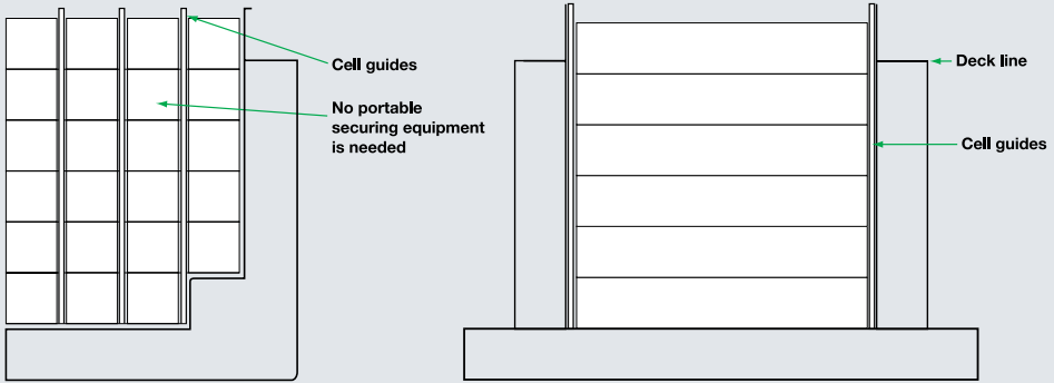
40-FOOT CONTAINERS IN 40-FOOT CELL GUIDES
