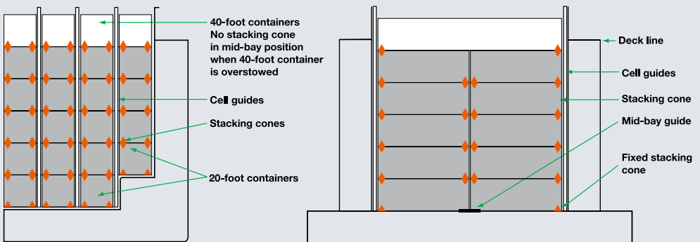
20-FOOT CONTAINERS IN 40-FOOT CELL GUIDES WITH 40-FOOT CONTAINERS STOWED ABOVE
